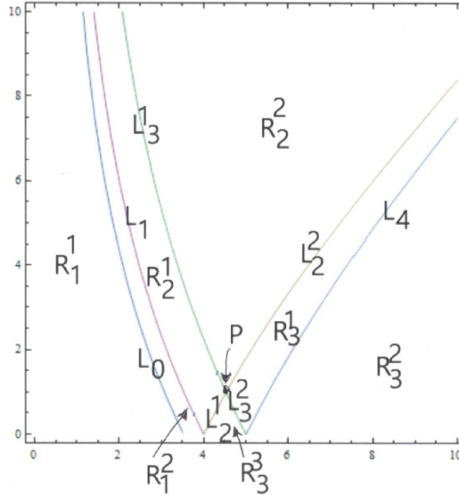
FIGURE 2. Bifurcation diagram on the local phase portraits at the equilibrium points in the parameter plane (a, b) with a and b positive.
