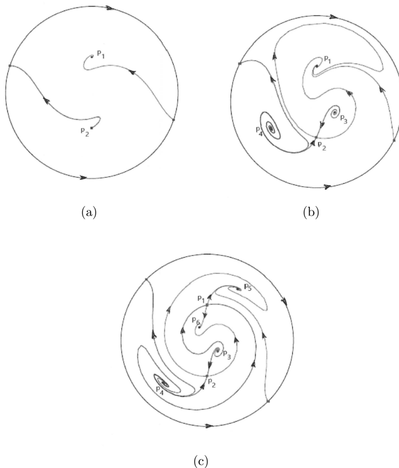
FIGURE 4. (a) The phase portrait of system (2) for (a, b) = (6, 2) . (b) The phase portrait of system (1) when (a, b) = (4, 8) . (c) The phase portrait of system (1) for some values of the parameters (a, b) = (2, 1) .
