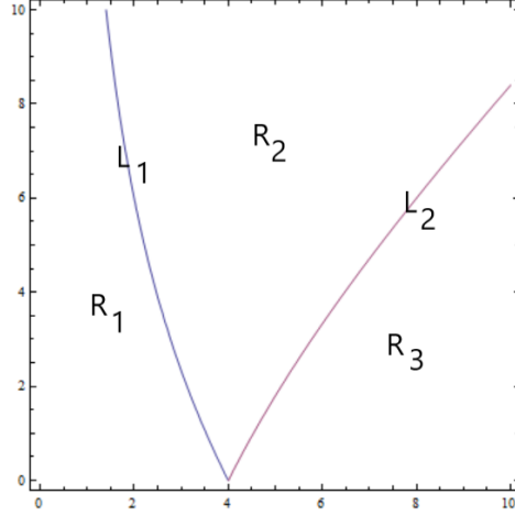
FIGURE 1. Bifurcation diagram on the number of equilibrium points in the parameter plane (a, b) with a and b positive.
