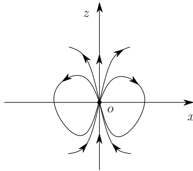
FIGURE 3. Local phase portrait of system (19) at the origin.
