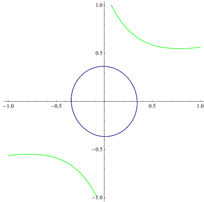
FIGURE 3. The limit cycle of system (29) and the boundary of the region \mathcal{R} .
