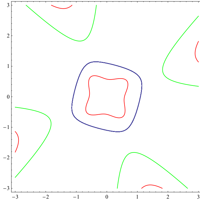
FIGURE 5. The limit cycle of system (34), the oval \sigma_\lambda and the boundary of the region \mathcal{R} when \lambda = -1 .
