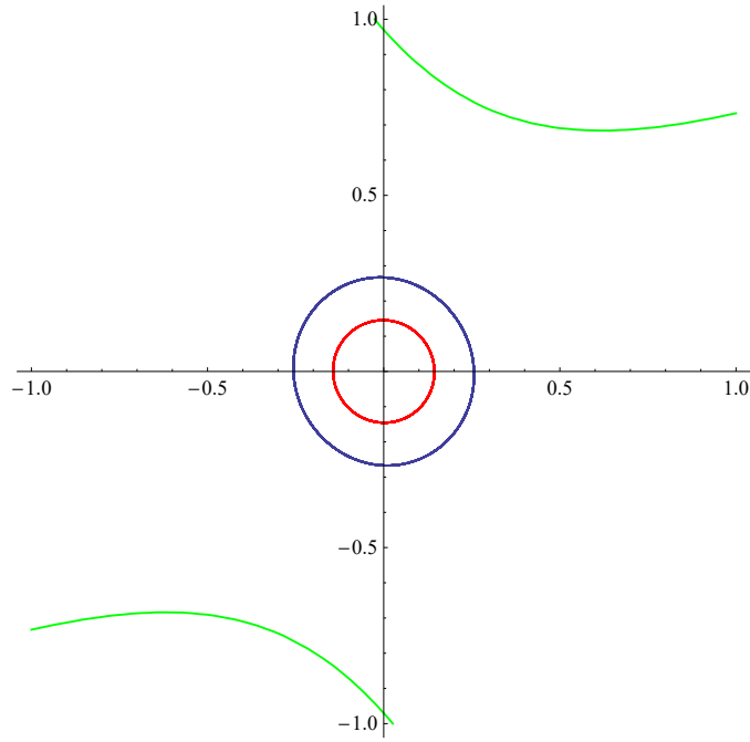
FIGURE 1. The two limit cycles of system (27) and the boundary of the region \mathcal{R} .
