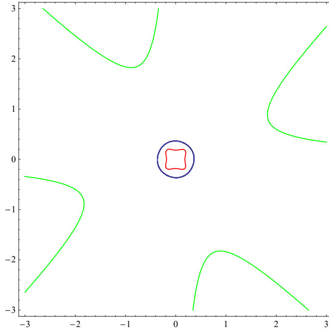
FIGURE 4. The limit cycle of system (34), the oval \sigma_\lambda and the boundary of the region \mathcal{R} when \lambda = -1/10 .
