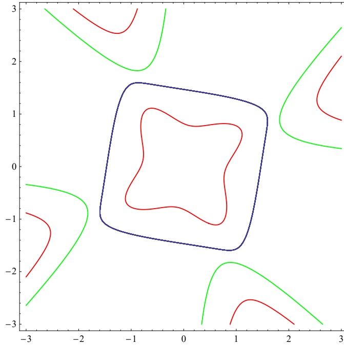
FIGURE 6. The limit cycle of system (34), the oval \sigma_\lambda and the boundary of the region \mathcal{R} when \lambda = -2 .
