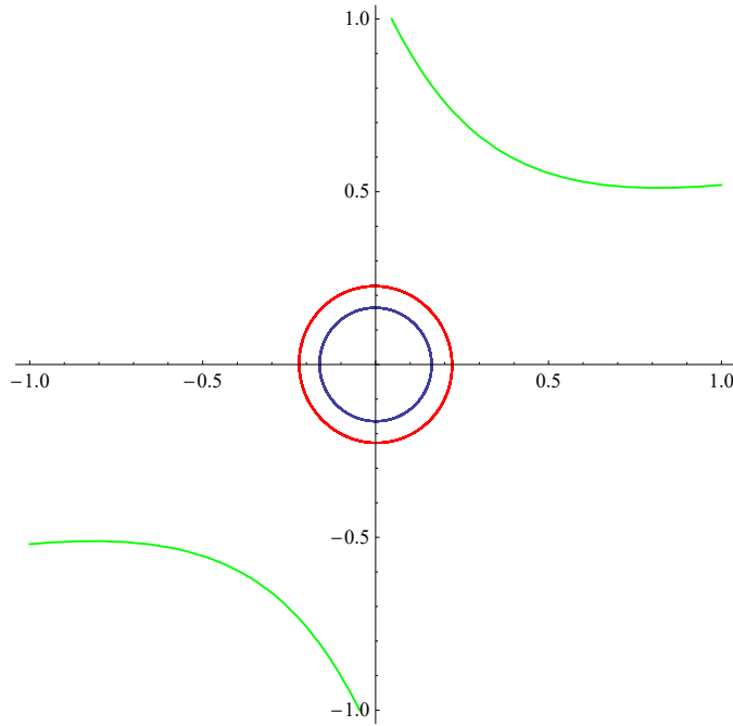
FIGURE 2. The two limit cycles of system (28) and the boundary of the region \mathcal{R} .
