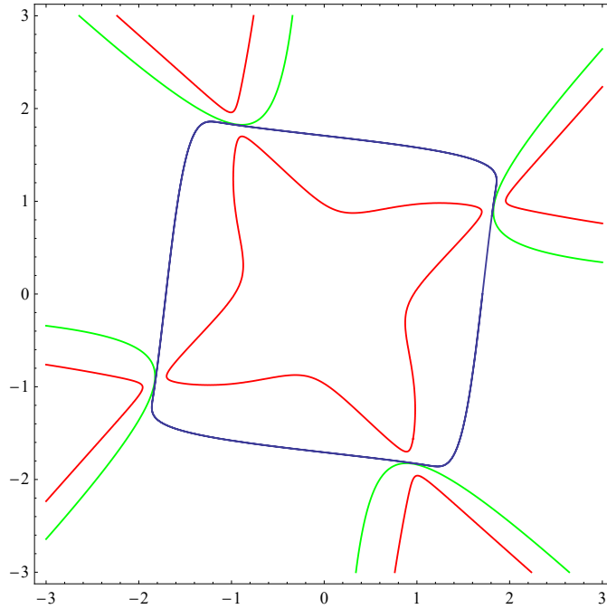
FIGURE 7. The limit cycle of system (34), the oval \sigma_\lambda and the boundary of the region \mathcal{R} when \lambda = -2.8 .
