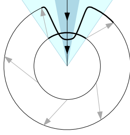
FIGURE 2. Action of f on a circle r = c (inner circle) represented schematically by arrows, sectors \widehat{I} (light) and \widehat{J} (dark) are shadowed, the attracting f -invariant ray ( \theta = \bar{0} ) is depicted vertical.
