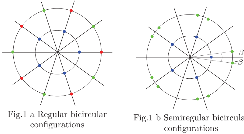
FIGURE 1. Examples of bicircular configurations
