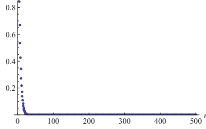
FIGURE 8. Plot of m_2(b_n) .
