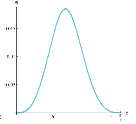
Fig. 10b The plot of m(a_4(\beta), \beta) for n = 3
