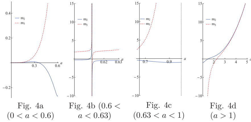
FIGURE 4. Plot of the masses m_2 (continuous line) and m_3 (dashed line) for n = 4 .
