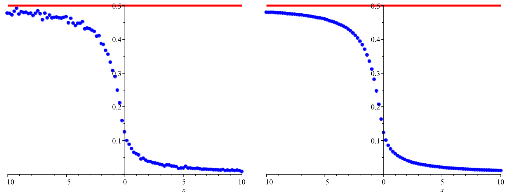
Fig. 3. Numerical approximation of P^+(\alpha) obtained with Monte Carlo simulation with samples of 10^4 (left panel) and 10^6 (right panel) points for 101 equidistributed values of \alpha in [-10, 10] .
