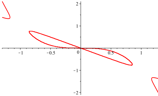
Fig. 2. An example of set \{V(x, y) = 0\} with two bubbles and sharing a common point.
