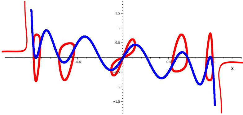
Fig. 1. An example of set \{V(x, y) = 0\} , in red, together with its symmetry curve \mathcal{C} , in blue. It has 6 bubbles, with two colliding ones.
