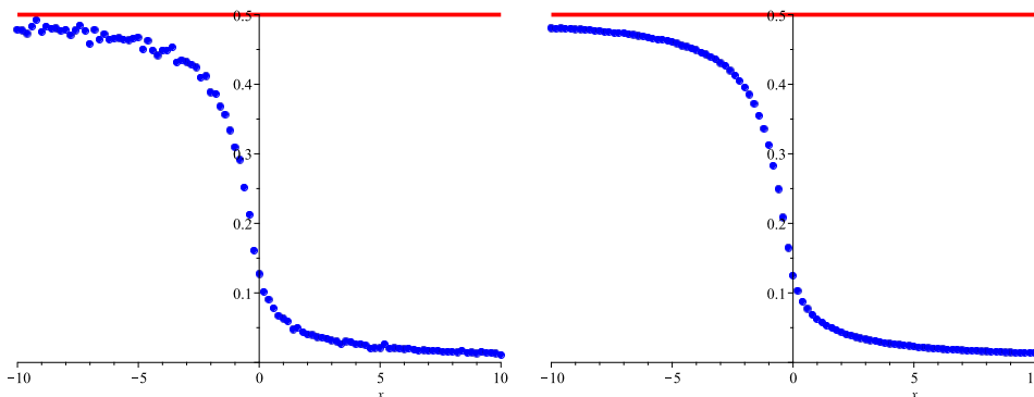
FIGURE 3. Numerical approximation of P^+(\alpha) obtained with Monte Carlo simulation with samples of 10^4 (left one) and 10^6 (right one) points for 101 equidistributed values of \alpha in [-10, 10] .
