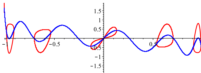
FIGURE 1. An example of set \{V(x, y) = 0\} , in red, together with its symmetry curve \mathcal{C} , in blue. It has 6 bubbles, with two colliding ones.
