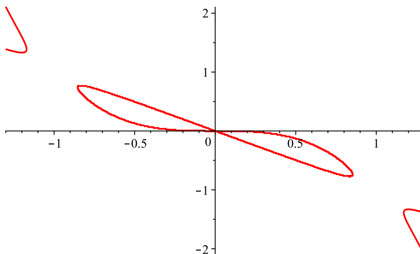
FIGURE 2. An example of set \{V(x, y) = 0\} . It has 2 bubbles, sharing a common point.
