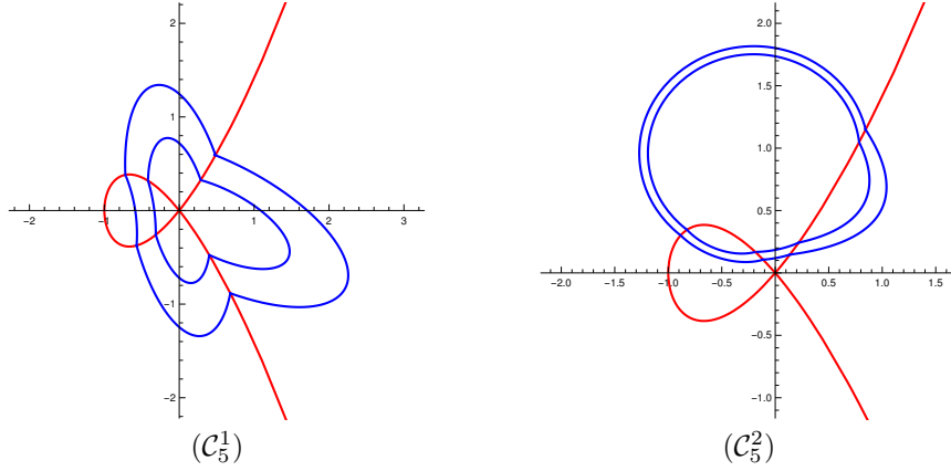
FIGURE 6. The two limit cycles of the discontinuous piecewise linear differential system ( \mathcal{C}_5^1 ) for (15)–(17), and ( \mathcal{C}_5^2 ) for (18)–(20) contained un three zones.
