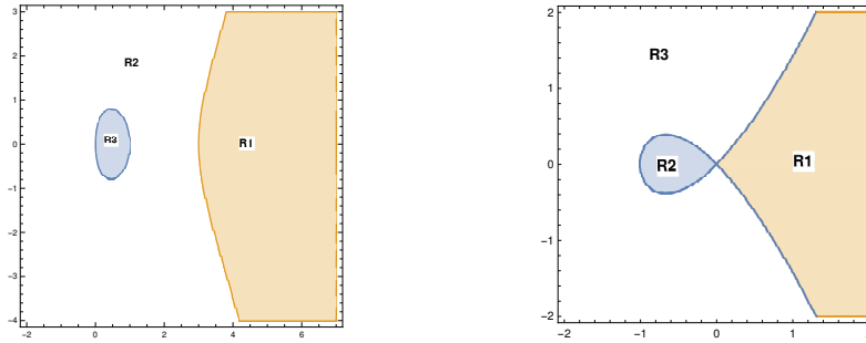
FIGURE 1. The three regions R_1 , R_2 and R_3 of the plane separated by the curves c_2 on the left and c_5 on the right.
