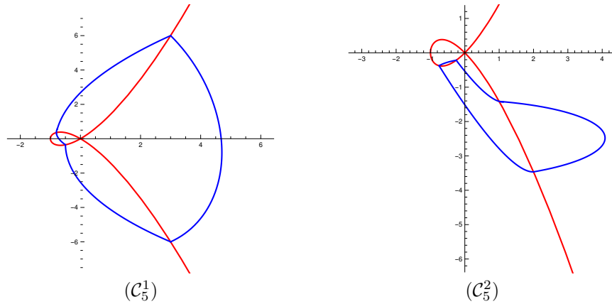
FIGURE 4. The unique limit cycle of the discontinuous piecewise linear differential system (\mathcal{C}_5^1) for (5)–(7), and (\mathcal{C}_5^2) for (9)–(11) contained in three zones.
