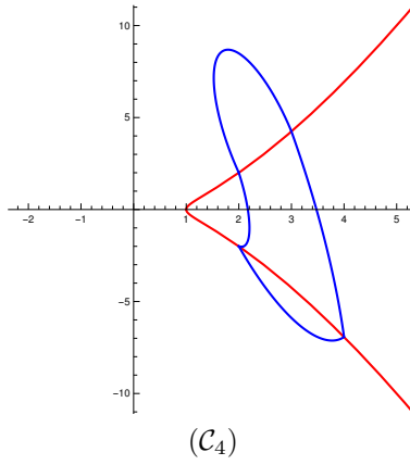
FIGURE 12. The unique crossing limit cycle of the discontinuous piecewise linear differential system (45)–(46) contained in two zones.
