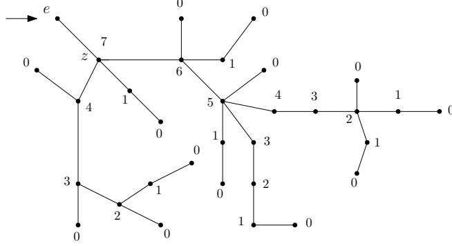
FIGURE 9. Topological induction
