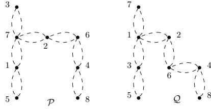
FIGURE 3. Two 8-periodic simplicial patterns \mathcal{P} and \mathcal{Q} .
