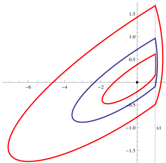
FIGURE 1. The first example with 3 limit cycles.
